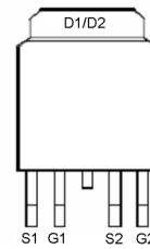
TO252-4L
