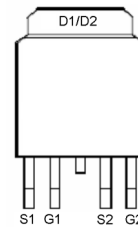
TO252-4L
