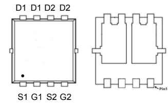
DFN3X3-8L
