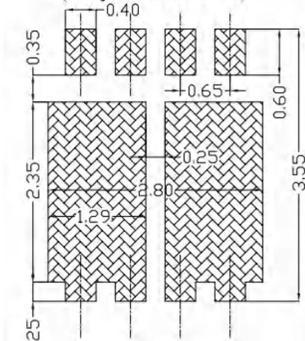
Land Pattern (Only for Reference)
