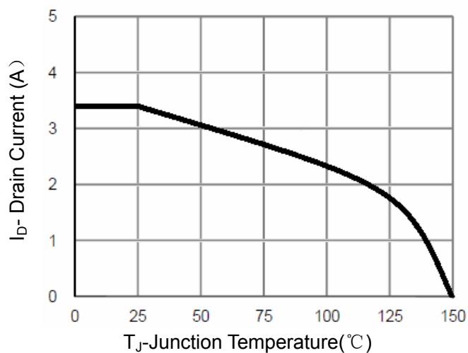
Figure 4 Drain Current
