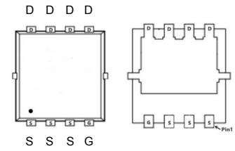
DFN5X6-8L
